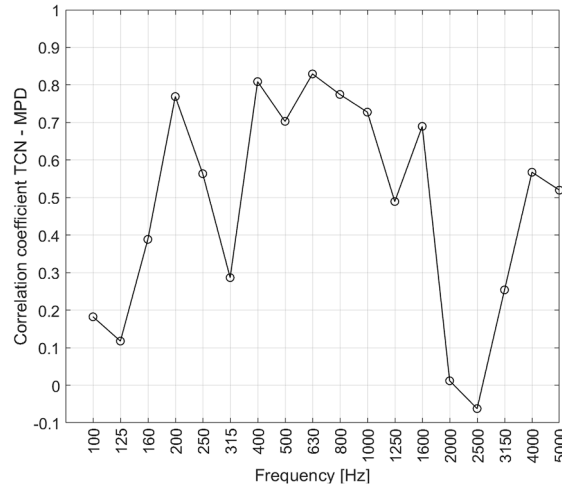
Fig. 7. Correlation coefficient between TCN and MPD.
