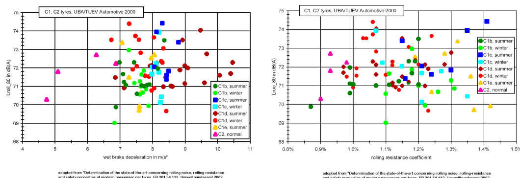
Figure 16 Correlation between low noise, safety and rolling resistance characteristics for passenger car tyres
